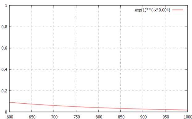
Fig. 4. Forecasting the tractor reliability after 600 mth of operation
