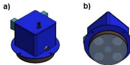
Fig. 1. Model of improved seed distribution uniformity collector for pneumatic seeding [7]
